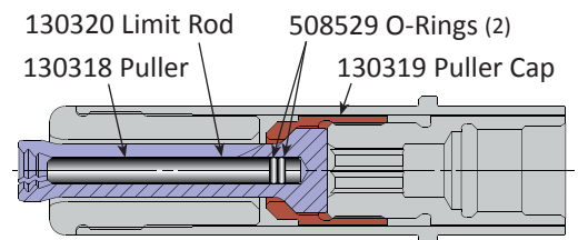
130360 Puller Assembly components
